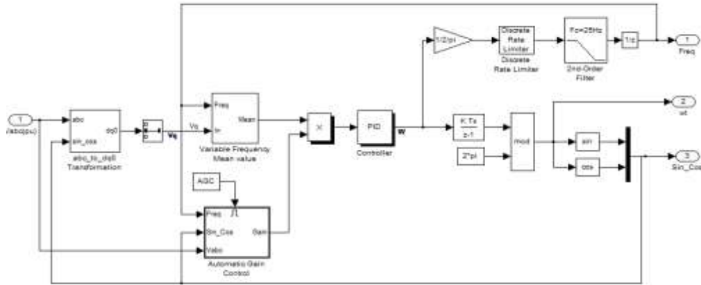
Fig Discrete phase PLL
